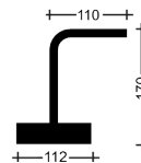
Single layer element ø 12mm
